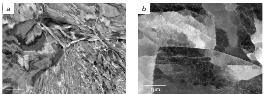
Fig. 5: Channeling contrast imaging of dislocation networks in highly deformed stainless steel. The sample is imaged at 30 kV electron beam energy. (a) Strong crystalline orientation changes within the grains. (b) Dislocation networks formed by the deformation.
