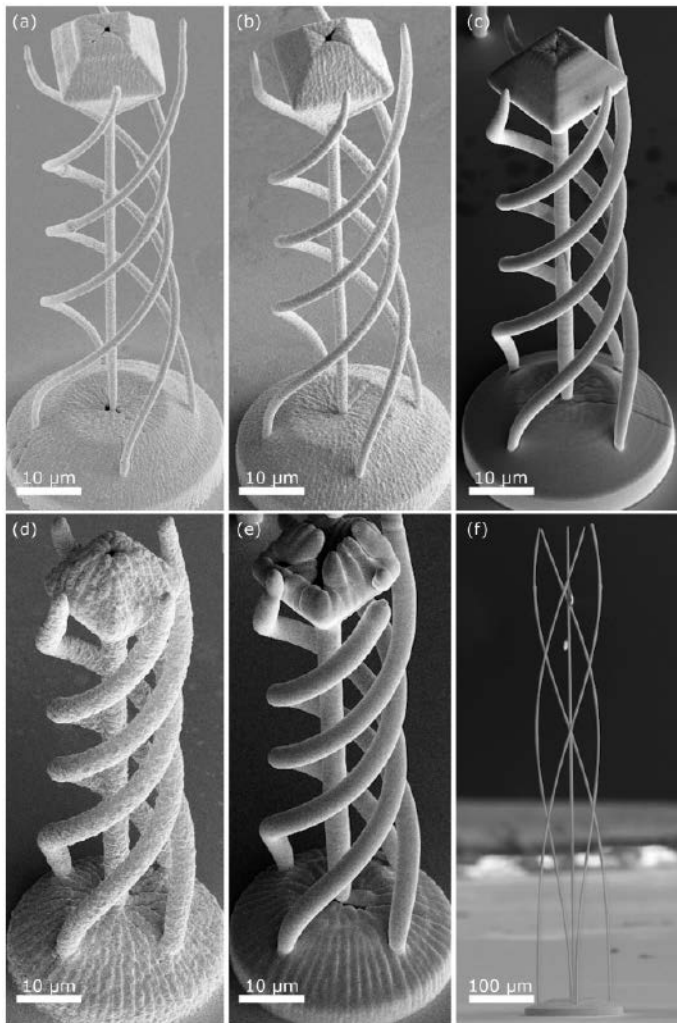
Fig. 4: A demonstration structure printed each time with a different tip aperture ranging in size from (a-e) 100 nm to 2 µm like in figure 3. (f) A larger 650 µm-tall structure was printed with a 300 nm tip, reaching an aspect ratio of 1:100 (strands).
