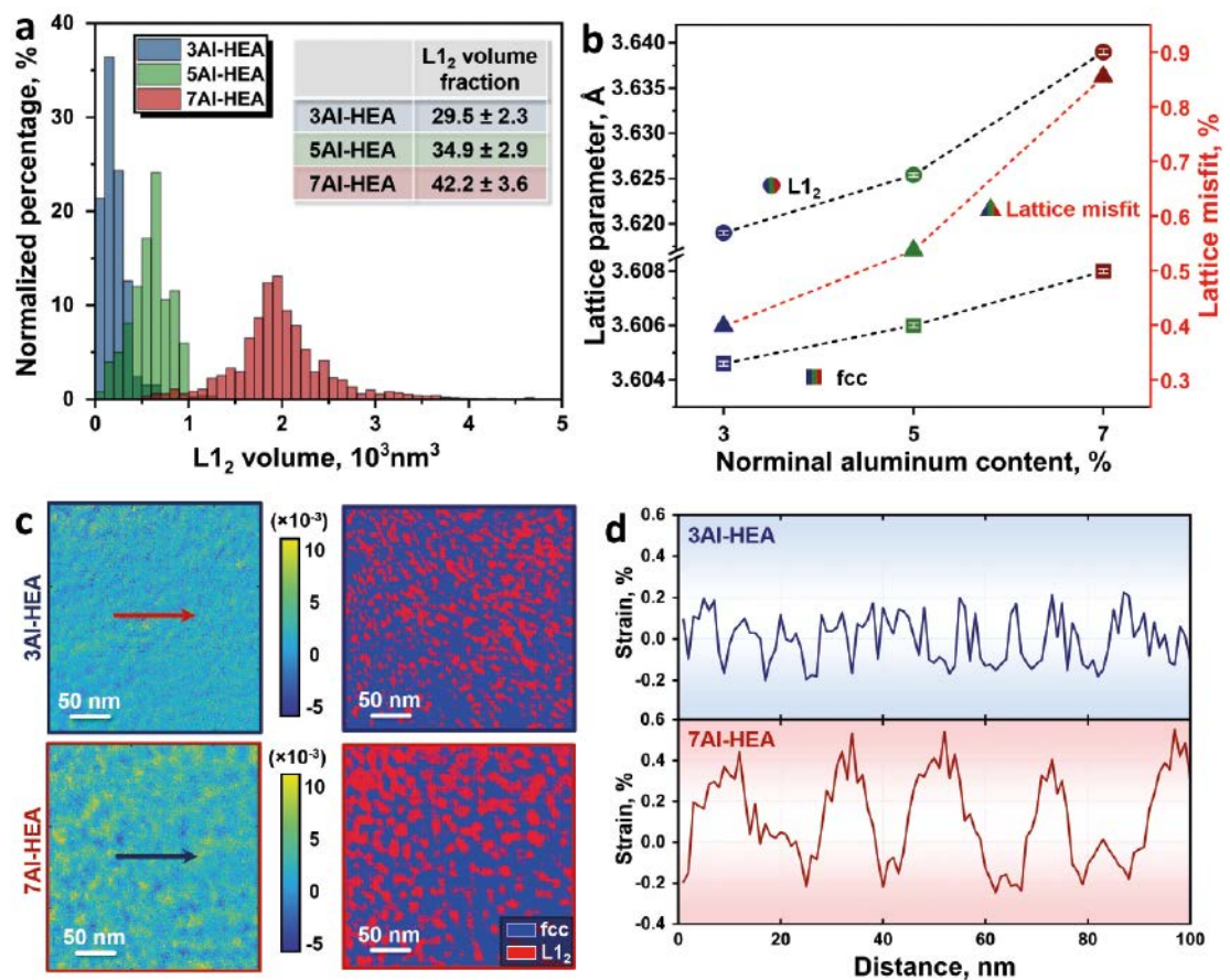
Fig. 4: Statistic volume distribution of the L 12 nanoprecipitates and quantitative lattice misfit and lattice strain in the HEAs. (a) Normalized percentage with respect to the single precipitate volume, the inset shows the overall volume fractions of L 12 precipitates. (b) Lattice parameter and lattice misfit of the L 12 and fcc phases. The lattice misfit ( \epsilon ) is calculated using the equation \epsilon = 2(\alpha_{L_{12}} - \alpha_{fcc}) / (\alpha_{L_{12}} + \alpha_{fcc}) , where \alpha_{L_{12}} and \alpha_{fcc} are the lattice parameters of the L 12 and fcc phases, respectively. [36] (c) Local strain distribution map and corresponding phase distribution map of the 3Al-HEA and 7Al-HEA. (d) 1D strain distributions along the arrows in (c).
