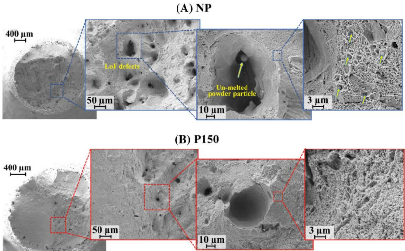
Fig. 4: Tensile fracture surfaces of laser beam powder bed fused (LB-PBF) 316L stainless steel (SS) specimens fabricated in (A) non-preheated (NP) and (B) preheated to 150°C (P150) conditions. The unmelted powder particles found in the lack of fusion (LoF) defects are shown by yellow arrows
