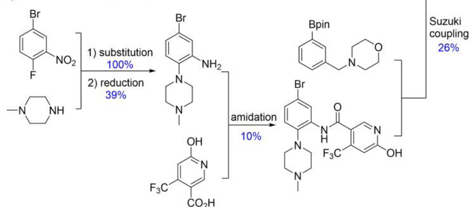
Figure 2. Two experimentally confirmed synthetic routes of OICR-9429. a) Synthetic route proposed by Chemata/Synthia™. Experimental yield was 60%. b) Literature route for OICR-9429. Reported yield was 1%.
