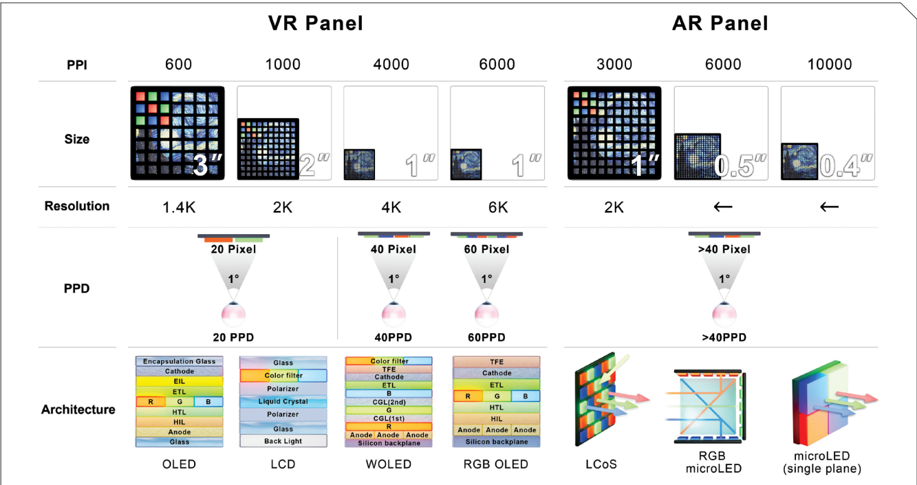
Fig. 5. The display technology trend for AR/VR applications. A red, green, and blue (RGB) micro-OLED display with high pixel density (~60 PPD) and monolithic RGB microLED displays with high brightness of more than 6,000 PPI will provide an immersive experience in VR or AR devices.
