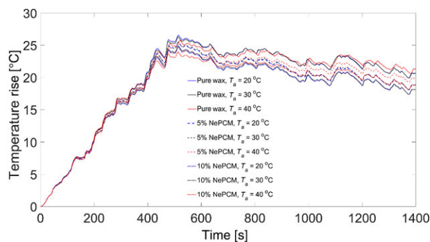
Figure 12. Variation of batteries average temperature under various PCM samples and air temperatures.
