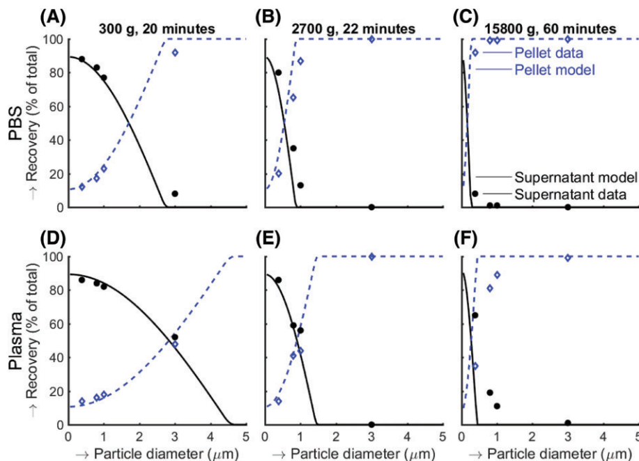
Figure 2. Centrifugation of beads diluted in PBS or plasma. The modeled bead recovery in pellet (blue dashed line) and supernatant (black, solid line) compared to measured bead recovery in pellet (open blue diamonds) and supernatant (closed black circles) for three centrifugation conditions. [Color figure can be viewed at wileyonlinelibrary.com ]
